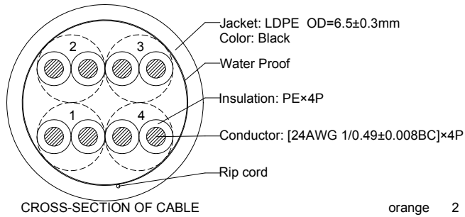
CROSS-SECTION OF CABLE
